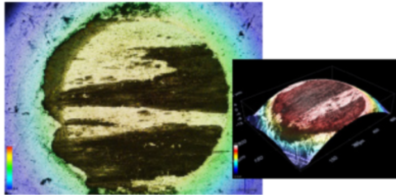
Figure 2. 3D topography acquired using Confocal technique (2D and 3D view). Transfer layers evolved on the worn ball cap of a steel ball during friction against W-C:H coating in humid air and flowing nitrogen atmospheres.
