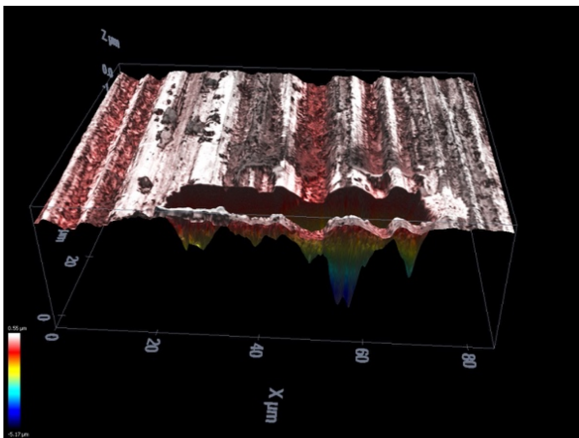
Figure 4. Topography of the scratched area in the contact zone with the transfer layer filling the grooves; the groove profiles were also revealed by a FIB cross section.
